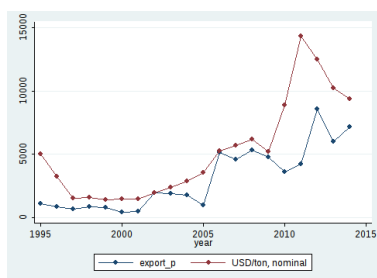
(a) Antimony
