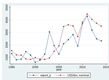
(e) Copper
