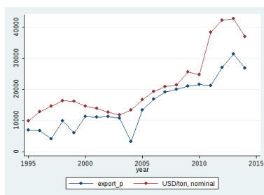
(f) Iodine
