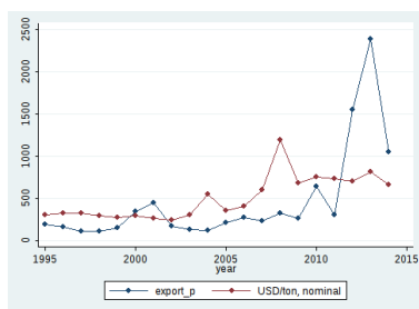
(g) Manganese
