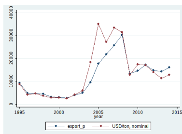
(h) Molybdenum
