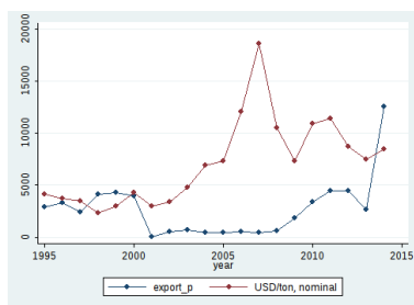
(i) Nickel
