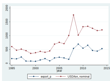
(c) Chromium
